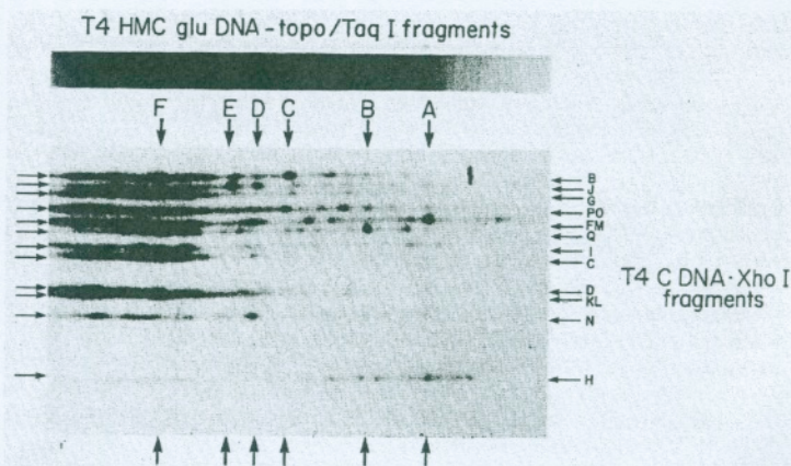
Figure 10. Hybridization of radioactive T4 topoisomerase cleavage fragments of native T4 DNA to an XhoI restriction digest of C T4 DNA. To prepare conveniently enough radioactive topoisomerase cleavage fragments for this procedure, intact T4 DNA containing HMC glu was treated with topoisomerase in the presence of oxolinic acid, and the reaction was terminated by adding SDS to 0.2%. Following proteinase-K treatment (to remove the covalently attached topoisomerase), the reaction products were subjected to gel filtration to remove SDS, and the recovered DNA was labeled at the 3' end with T4 DNA polymerase (O'Farrell et al. 1980), which thereby specifically labels the positions of topoisomerase cleavage, as well as the randomly placed ends of the circularly permuted T4 genome. This labeled DNA was then cleaved with TaqI to generate discretely sized fragments in high yield for hybridization. The band pattern of cleavage fragments generated using this procedure is very similar to that obtained using the method described in Fig. 9 (data not shown). The Southern cross-blot was prepared as described by Wensink et al. (1979), with the following exceptions. The first dimension was a horizontal 0.6% agarose gel loaded with 10–15 µg of an (unlabeled) restriction digest of C T4 DNA. The gel was stained with ethidium bromide and photographed to record the positions of the restriction fragment bands. The DNA was then denatured and transferred to nitrocellulose as described previously (Wensink et al. 1979). The second dimension was a horizontal 1.2% agarose gel, loaded with radioactively labeled topoisomerase/ TaqI cleavage fragments. A segment of this gel was dried down directly for autoradiography to determine the positions of the radioactive cleavage fragments, and the rest of the gel was transferred under hybridization conditions to nitrocellulose (rotated 90° with respect to the first gel). The gel at the top shows the radioactive cleavage fragments without hybridization, and the major bands are labeled A through F in order of increasing electrophoretic mobility. Arrows indicate the positions of unlabeled XhoI restriction fragments of C T4 DNA (designations are those of O'Farrell et al. [1980]). The small XhoI fragment A did not show any significant hybridization and is not shown, and XhoI fragment E ran off the gel.
