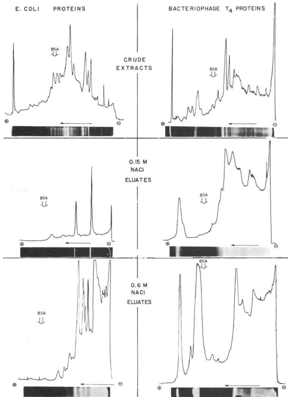
FIGURE 5. Polyacrylamide gel electrophoresis of ^{35}\text{S} -labeled DNA-binding proteins. Samples of 0.10 ml of the peak fractions from Fig. 4 and an aliquot of dialyzed extract were analyzed in the pH 8 gel system of Jovin et al. (1964), using 5 mm I.D. \times 7 cm gels. To facilitate subsequent drying, the bottom gel composition was changed to 7.5% acrylamide, 0.10% bisacrylamide. Gels were fixed and stained for 24 hr in 10% TCA plus 1/20th saturated Coomassie Brilliant Blue R250 (Colab Laboratories, Chicago). Less than 0.5 \mu\text{g} of protein per band could be readily seen, even without destaining. The gels were then dried and autoradiographed (Fairbanks et al., 1965). Joyce-Loebl tracings of over-exposed films are shown in order to maximize detail; tracings of less exposed films are given in Fig. 6. Exposure times were 1 to 5 days. Band patterns which are very similar, but not identical, to those above were obtained in experiments in which the T4 native DNA-cellulose was replaced by either calf thymus native or denatured DNA-cellulose, and when phase-extracted extracts (Fig. 3) were chromatographed in the presence of 0.01 M \text{MgCl}_2 . It is therefore clear that the majority of DNA-binding proteins neither show an absolute specificity for a particular species of DNA, nor require \text{Mg}^{++} for their binding.
