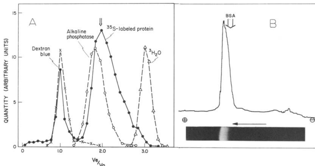
FIGURE 13. Characterization of 32 protein on Sephadex G-200. (A) Details were as described in Fig. 7, except that the 2.0 M NaCl peak from a denatured DNA-cellulose fractionation (Fig. 10A) was applied to the Sephadex column. About 70% of the ^{35}\text{S} -labeled protein was recovered. Alkaline phosphatase was assayed by the standard colorimetric assay (Garen and Levinthal, 1960) with 0.1 mM \text{ZnCl}_2 added. (B) This polyacrylamide gel autoradiograph of the peak Sephadex fraction (arrow in (A) above) was obtained by the procedures outlined in Fig. 5. It proves that the protein in these fractions is indeed 32 protein, and thus substantiates the results in Fig. 7.
