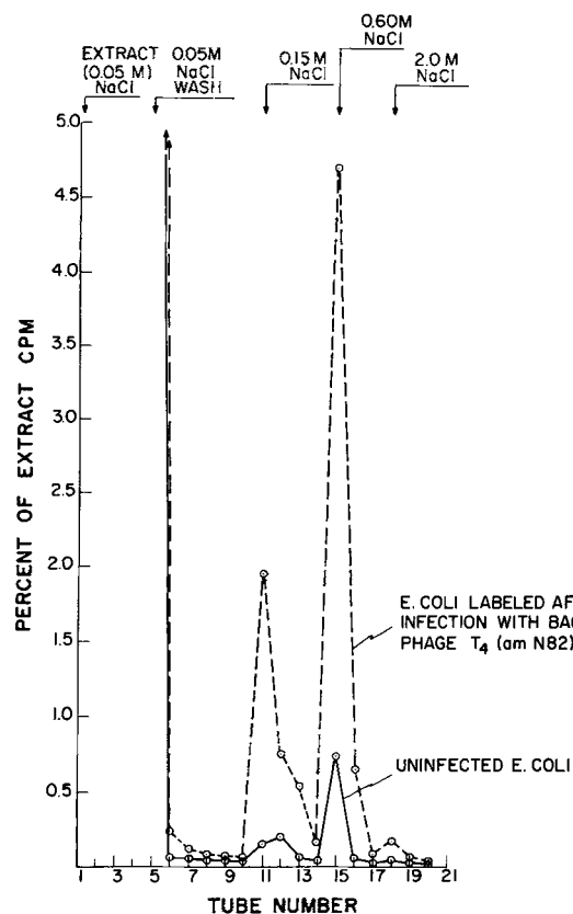
FIGURE 3. Purification of E. coli RNA polymerase on calf-thymus native DNA-cellulose. After sonication of 2 g of RNase - cells as described in Fig. 2, the sonicate was made 5 M in NaCl and centrifuged at low speed. To a total volume of 10 ml of supernatant, 0.6 g powdered Carbowax 6000 (Union Carbide Chemicals) and 0.4 g Dextran 500 (Pharmacia) were added. The polymers were dissolved by mixing at 4°, and two phases of approximately equal volume were separated by a 10 min centrifugation at 10,000 × g . The polyethylene glycol-rich top phase was withdrawn and dialyzed. All subsequent details were identical to those in Fig. 2, except that the 5 ml of dialyzed extract (~8 mg/ml protein) was chromatographed without further dilution on a 1 ml DNA-cellulose column containing 0.56 mg of native calf thymus DNA (Worthington Biochemical). Fractions of 0.5 ml were collected at 15 min intervals. The count/min given are for 1 μl of enzyme in 50 μl of reaction mixture (Fig. 2), with incubation for 5 min at 37°. A variable fraction of the RNA polymerase activity precipitates in the phase system; consequently, somewhat less than one-half of the initial sonicate activity is normally recovered by this procedure. In preliminary studies of 0.60 M NaCl eluates from similar columns, nearly complete binding of DNA methylase activity from strain MRE600 has been observed using the assay of Gold and Hurwitz (1964). Substantial E. coli deoxy-ribonuclease activity is also bound, although the major portion of this activity passes through the column (B. Alberts, unpubl. experiments).
