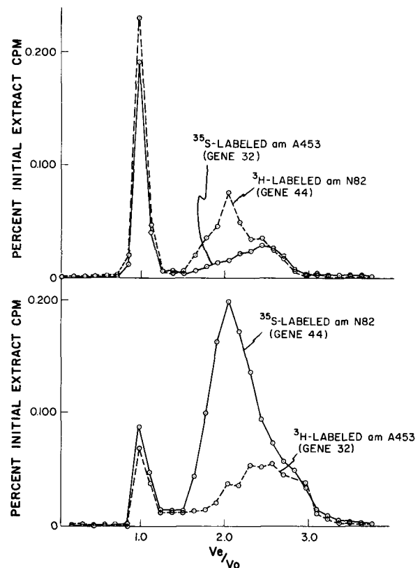
FIGURE 7. Sephadex G-200 fractionation of labeled (4 to 8 min, 25°) bacteriophage T4-induced, DNA-binding proteins. A 40 cm \times 0.8 cm I.D. column of Sephadex G-200 at 4° was equilibrated with a buffer consisting of 0.10 M NaCl, 0.001 M Na 2 EDTA, 0.001 M mercaptoethanol, 0.02 M Tris-HCl, pH 8.1, 10% glycerol and 500 \mu\text{g}/\text{ml} BSA. Aliquots (0.3 ml) of 0.60 M NaCl DNA-cellulose eluates, obtained as described in the text, were washed through the column with this buffer at 2 ml/hr. The fractions obtained were counted in Brays-Cab-O-Sil scintillation fluid. The results shown have been corrected for channel overlap between the two radioisotopes; only 25–30% of the labeled protein applied to the column was recovered.
