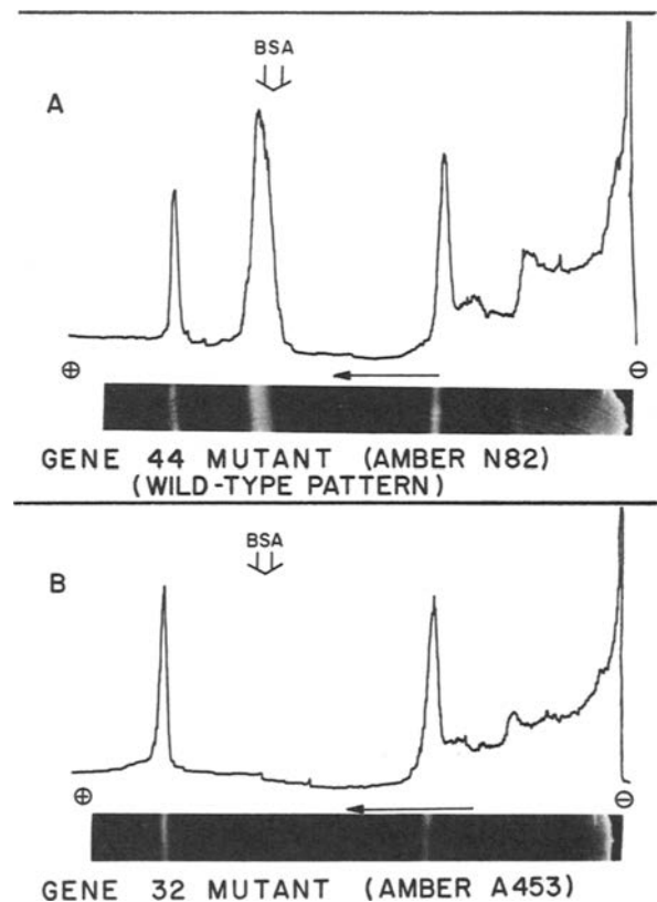
FIGURE 6. Polyacrylamide gel pattern of DNA-binding proteins from E. coli infected with amber mutants of bacteriophage T4. Experimental details are those described in Figs. 4 and 5. (A) 0.60 M NaCl eluate of extract from cells infected with T4 amN82 (gene 44). (B) 0.60 M NaCl eluate of extract from cells infected with T4 amA453 (gene 32). The gel patterns for the amA453 crude extract and 0.15 M NaCl eluate were indistinguishable from those given in Fig. 5. The single band difference in the 0.60 M eluate was maintained in the patterns obtained when urea-denatured samples were run through polyacrylamide gels containing 8 M urea (Jovin et al., 1964).
