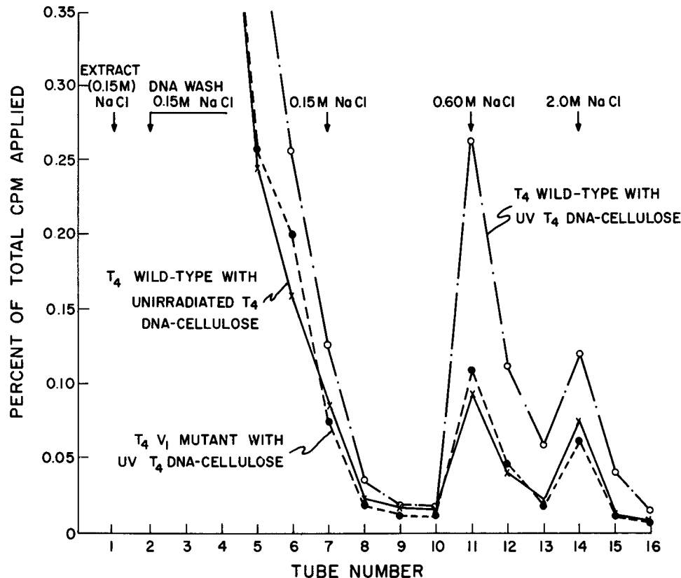
FIGURE 14. Specific binding of T4-induced proteins to UV-irradiated T4 DNA-cellulose. Native T4 DNA (500 ml of 50 \mu\text{g}/\text{ml} ) was irradiated with constant mixing in a quartz cylinder of 8 cm diameter, surrounded by 3 germicidal lamps, type G15T8. These were placed a distance of 7 cm from the cylinder axis. The apparatus was calibrated by uridine bleaching (McLaren and Shugar, 1964); 2.5 quanta were absorbed per DNA nucleotide in the 1 min of irradiation used. Reference to the data of Wulff (1963) indicates that 5% of the thymine bases in this DNA were dimerized. After concentration by alcohol precipitation and dialysis, both the irradiated T4 DNA and an aliquot of the initial sample were adsorbed to cellulose under identical conditions. The three DNA-cellulose columns shown were run simultaneously, with the only variables being those indicated. Extracts from 5 \times 10^{10} infected cells were made as previously described in Fig. 4, except that the DNase treatment was omitted and the dialyzed extract was clarified by centrifugation for 30 min at 38,000 rpm. One hr before loading the columns, the extract was diluted with 2 volumes of 'rinse buffer' containing 250 \mu\text{g}/\text{ml} sonicated, native T4 DNA plus 250 \mu\text{g}/\text{ml} of sonicated, heat-denatured T4 DNA. This same DNA-containing 'rinse buffer' was used for the DNA wash. Fractions of 0.5 ml were collected at 15 min intervals. All DNA-cellulose columns were 0.75 packed ml and contained 0.4 mg of DNA.
