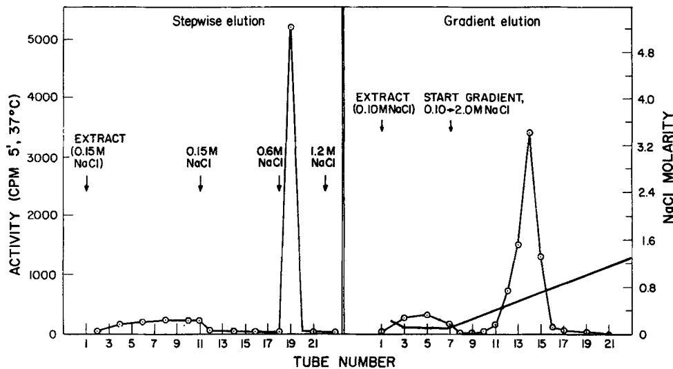
FIGURE 3. Purification of E. coli RNA polymerase on calf-thymus native DNA-cellulose. After sonication of 2 g of RNase - cells as described in Fig. 2, the sonicate was made 5 M in NaCl and centrifuged at low speed. To a total volume of 10 ml of supernatant, 0.6 g powdered Carbowax 6000 (Union Carbide Chemicals) and 0.4 g Dextran 500 (Pharmacia) were added. The polymers were dissolved by mixing at 4°, and two phases of approximately equal volume were separated by a 10 min centrifugation at 10,000 × g . The polyethylene glycol-rich top phase was withdrawn and dialyzed. All subsequent details were identical to those in Fig. 2, except that the 5 ml of dialyzed extract (~8 mg/ml protein) was chromatographed without further dilution on a 1 ml DNA-cellulose column containing 0.56 mg of native calf thymus DNA (Worthington Biochemical). Fractions of 0.5 ml were collected at 15 min intervals. The count/min given are for 1 μl of enzyme in 50 μl of reaction mixture (Fig. 2), with incubation for 5 min at 37°. A variable fraction of the RNA polymerase activity precipitates in the phase system; consequently, somewhat less than one-half of the initial sonicate activity is normally recovered by this procedure. In preliminary studies of 0.60 M NaCl eluates from similar columns, nearly complete binding of DNA methylase activity from strain MRE600 has been observed using the assay of Gold and Hurwitz (1964). Substantial E. coli deoxy-ribonuclease activity is also bound, although the major portion of this activity passes through the column (B. Alberts, unpubl. experiments).
