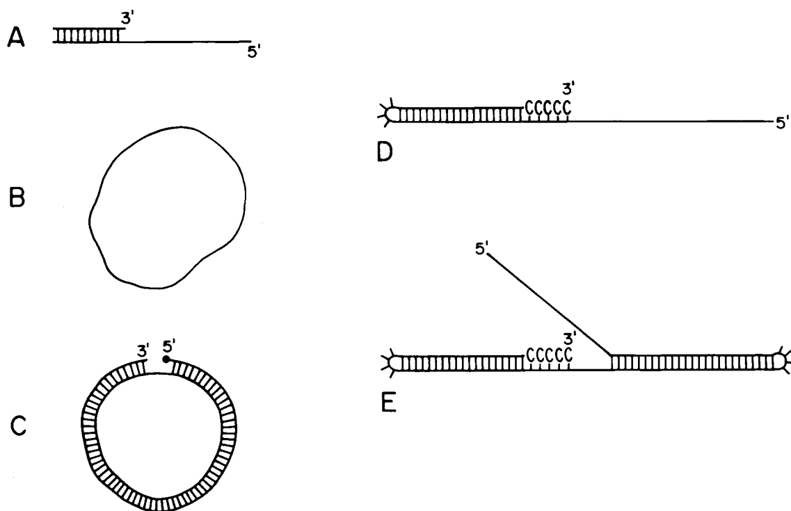
Figure 6. Some special types of DNA molecules that have been useful for studying DNA replication mechanisms. The molecules shown in D and E are defined-sequence molecules that have been chemically synthesized. In addition to having structures that mimic aspects of a DNA replication fork, they contain a contiguous run of C residues at their 3' ends; these are necessary to keep the T4 DNA polymerase in place in the presence of dCTP (M. Munn and M. Urdea, unpubl.).
