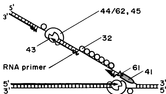
Figure 1. A two-dimensional view of the DNA replication fork of bacteriophage T4. The T4 DNA polymerase is the product of gene 43, and the gene-44/62 and -45 proteins that function with it are designated as "polymerase accessory proteins." The gene-32 protein binds to all of the single-stranded DNA at the fork; it is a helix-destabilizing protein, sometimes described as a "single-strand binding protein." The gene-41 protein is both a DNA helicase and a protein that is required, together with the gene-61 protein, for RNA primer synthesis on the lagging strand. The average length of the Okazaki fragments formed on the lagging strand is about 1500 nucleotides, both in vivo and in vitro.
