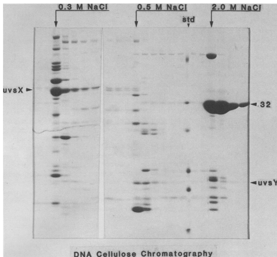
Figure 7. Analysis by SDS-polyacrylamide gel electrophoresis of the total proteins that bind to a single-stranded, calf thymus DNA cellulose column when a crude extract prepared from 200 g of T4-infected cells is loaded onto a 300-ml column in the presence of 0.1 M NaCl. Successive fractions have been analyzed in adjacent gel lanes, beginning with an elution with buffer containing 0.3 M NaCl, as indicated. The uvsX protein is the T4 RecA protein analog, and it has a molecular mass of about 40,000 daltons; the uvsY protein is likewise involved in genetic recombination in T4-infected cells, and it has a molecular mass of about 16,000 daltons (see Formosa and Alberts, this volume). Because the cells used for this fractionation were infected with T4 bacteriophage that were mutated in genes 33 and 55, they greatly overproduce the gene-32 protein (34,500 daltons). This gel was stained with Coomassie blue and therefore includes some E. coli host proteins. It represents the first step in the purification of the gene-61 protein, which is the doublet of two equally stained bands that migrate at about the same rate as the uvsX protein in the fractions just preceding the 0.5 M elution (M. Munn and J. Barry, unpubl.).
