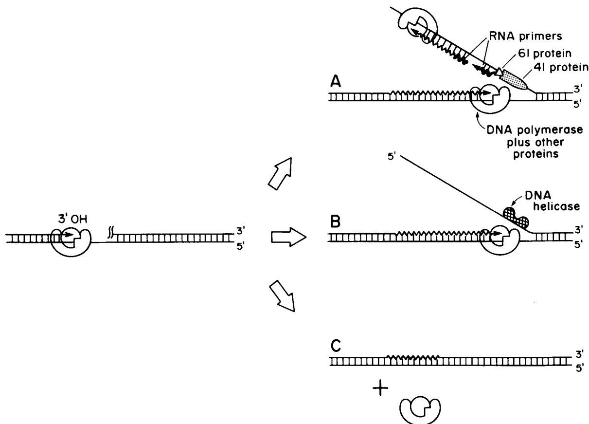
Figure 4. Diagram illustrating the results of assembling the T4 DNA polymerase into different replication protein complexes at different sites on the DNA. (A) A specific DNA sequence corresponding to a DNA replication origin directs the assembly of the T4 gene-4I protein onto the lagging strand. As a result, a true replication fork is established with both leading- and lagging-strand DNA synthesis. (B) Another type of specific DNA sequence (or structure) is proposed to have allowed a DNA polymerase molecule to coassemble into a protein complex that contains a DNA helicase different from the gene-4I protein. Because this DNA helicase is unable to participate in RNA primer synthesis, the DNA on the lagging strand remains single-stranded (see text). (C) A typical DNA repair reaction is shown, in which no DNA helicase is involved.
