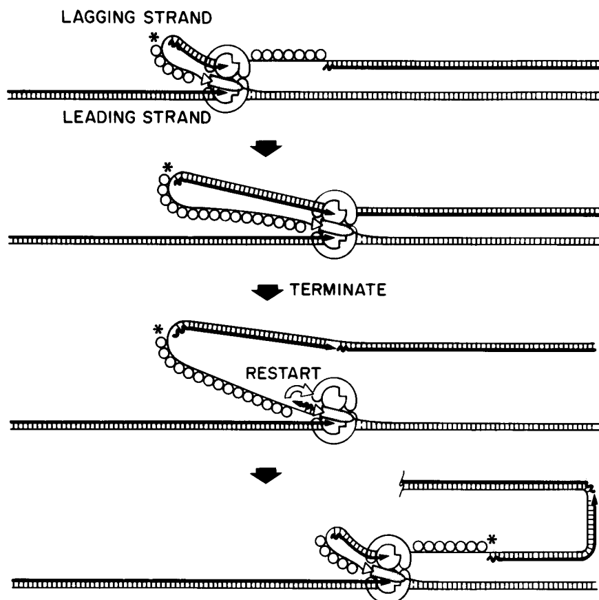
Figure 3. A model for DNA synthesis at a replication fork that allows the same DNA polymerase molecule to be repeatedly recycled to synthesize all of the Okazaki fragments on the lagging strand. The crucial step here occurs when the synthesis of each Okazaki fragment is completed. Rather than falling off of the entire fork assembly, the DNA polymerase molecule on the lagging strand remains bound to the assembly of replication proteins, letting go only of the DNA on the lagging strand. For the different symbols used to represent the T4 replication proteins, see Figs. 1 and 2.
