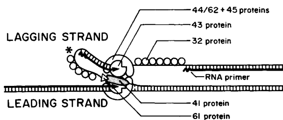
Figure 2. A schematic view of the seven proteins of the T4 DNA replication machine as they are thought to exist in an actual replication fork. The two-dimensional replication fork has been converted into the structure shown by folding the DNA on the lagging strand in such a way as to bring the DNA polymerase molecule on the lagging strand in close opposition to the DNA polymerase molecule on the leading strand. The lagging-strand DNA polymerase molecule is thereby held for many successive cycles of Okazaki fragment synthesis, as shown in Fig. 3.
