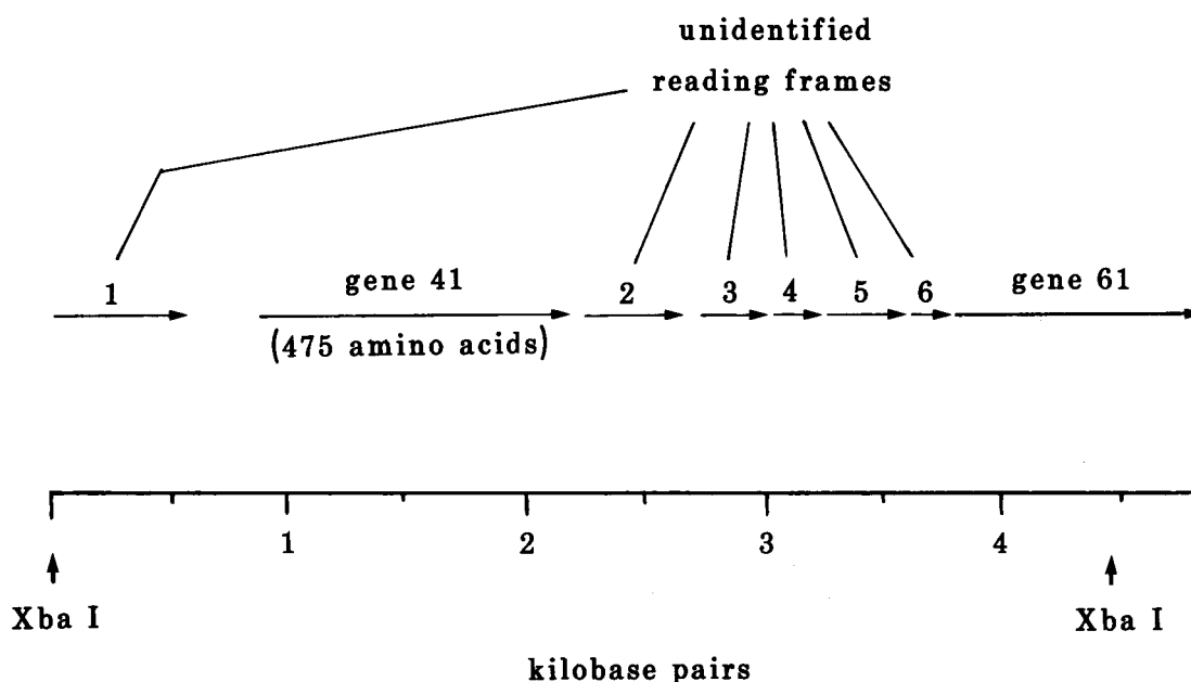
Figure 5. A sequenced early region of the T4 genome that contains five unidentified reading frames located between genes 41 and 61. This region is suspected of coding for small proteins, some of which interact with either the gene-41 or the gene-61 proteins and are involved in T4 DNA synthesis (M. Nakanishi et al., unpubl.).
